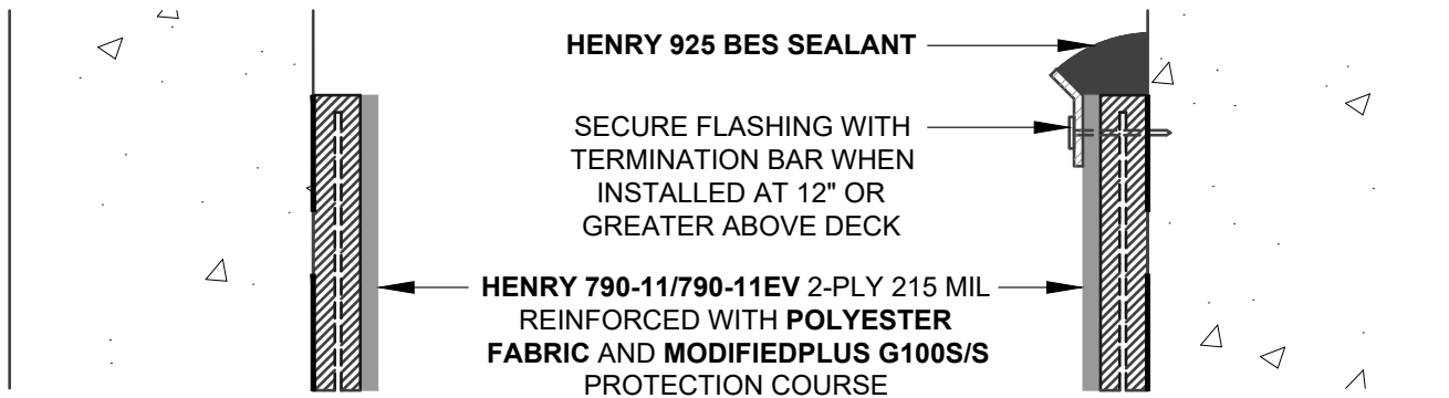
HOT RUBBERIZED ASPHALT N.T.S
