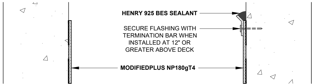
TORCH GRADE FLASHING N.T.S
