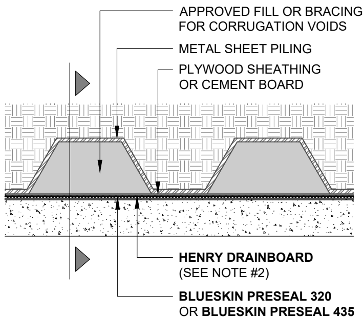
PLAN VIEW CUT THROUGH SHEET PILING
