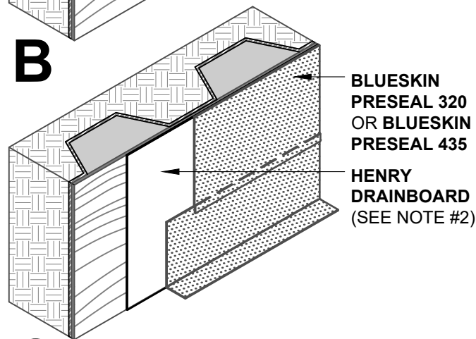
ISOMETRIC VIEW STEP-BY-STEP SHEET PILING
