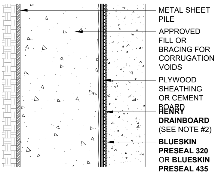
SECTION VIEW CUT THROUGH SHEET PILING
