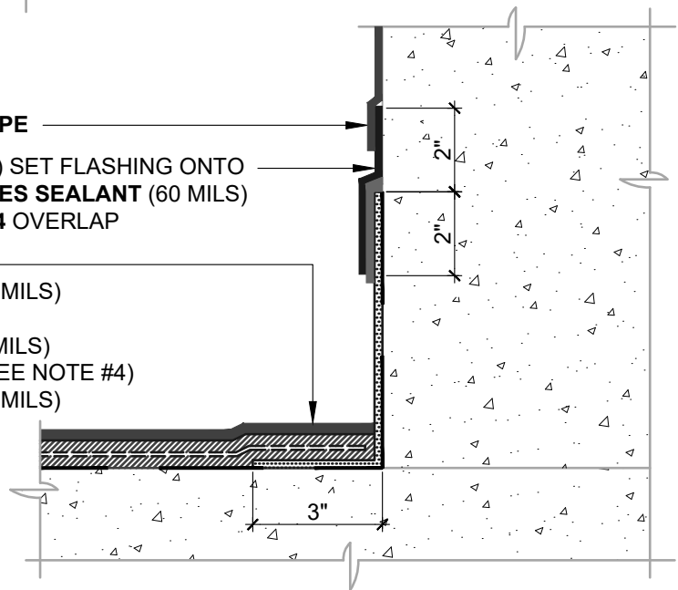
TORCH-GRADE FLASHING N.T.S
